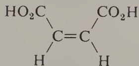
cis -Butene-dioic acid
